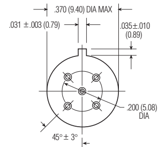
1MS/1MSD/1MSDD Header
